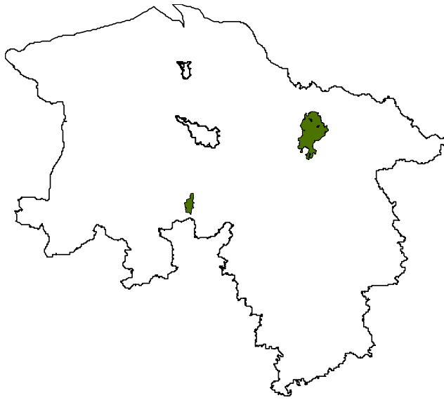
Fig. 1: The project's study plots are located in Lüneburger Heide nature reserve ( Calluna -heathlands on mineral soils; northeast) and Neustädter Moor nature reserve ( Calluna -heathlands on organic substrate; southwest).
