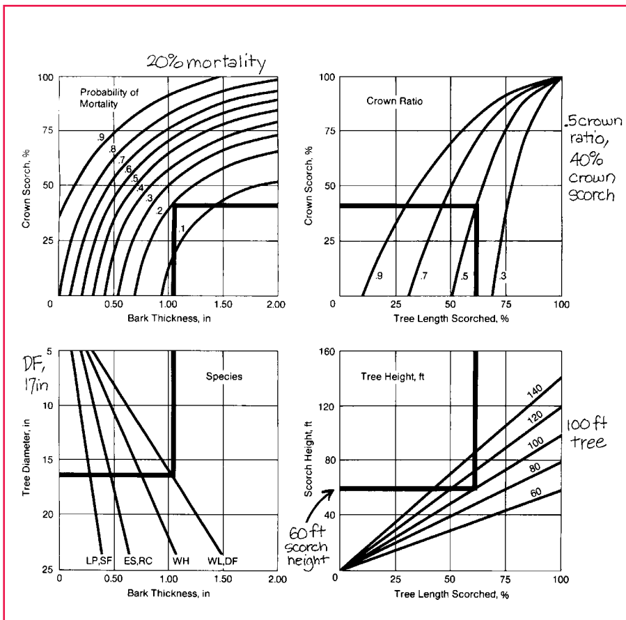
Figure 3 —This figure illustrates the use of the mortality nomogram to set scorch height limits for a prescribed underburn in which the target leaf trees are Douglas-fir, 17 inches (43 cm) in diameter at breast height, 100 feet (30 m) tall with a crown ratio of 0.5, and an acceptable mortality of 20 percent.
